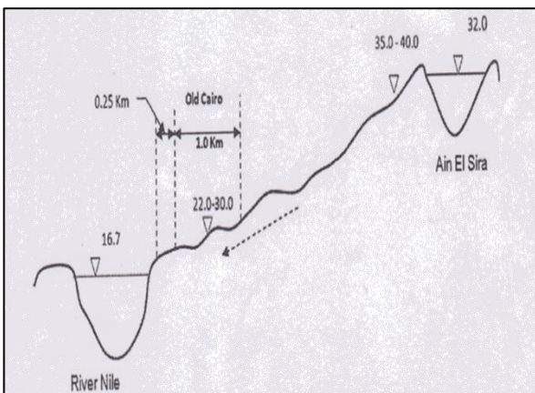
Figure 7: Sketch showing slopes and flow of untreated water
