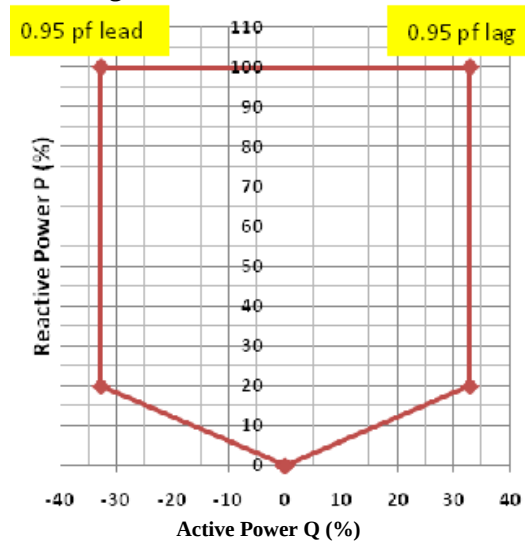
Fig. 15- P-Q Diagram for MSSPs
