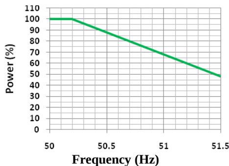
Fig. 14- Active Power Reduction Due To Over Frequency
