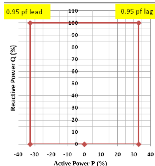
Fig. 16- P-Q Diagram for LSSPs
