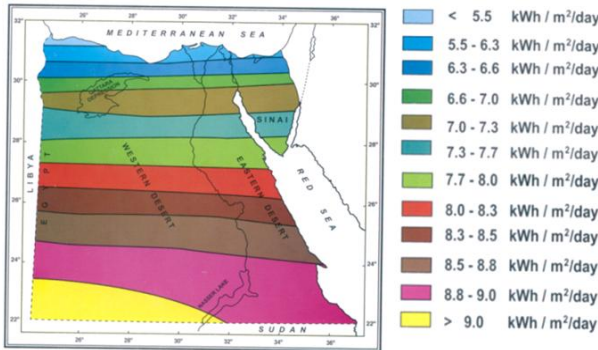
Fig. 2-Solar Atlas of Egypt [11]
