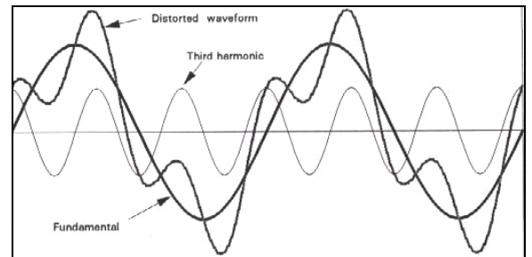
Fig. 12- Effect of Third Harmonic
