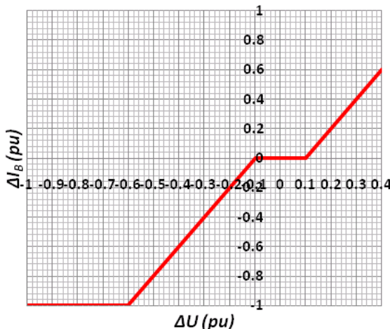
Fig.18: Current Injection During the Fault (k=2)
