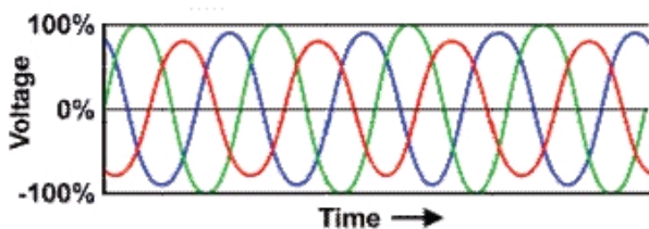
Fig. 13- Unbalanced Three-phase Voltages
