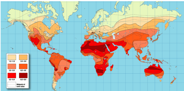
Fig. 1- Worldwide Annual Insolation [10]
